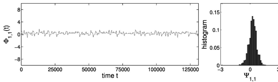
FIG. 2. Time evolution of \Phi_{1,1} for two independent Rössler systems, left graph. The distribution of \Psi_{1,1} , right figure, is showing a sharp peak.
