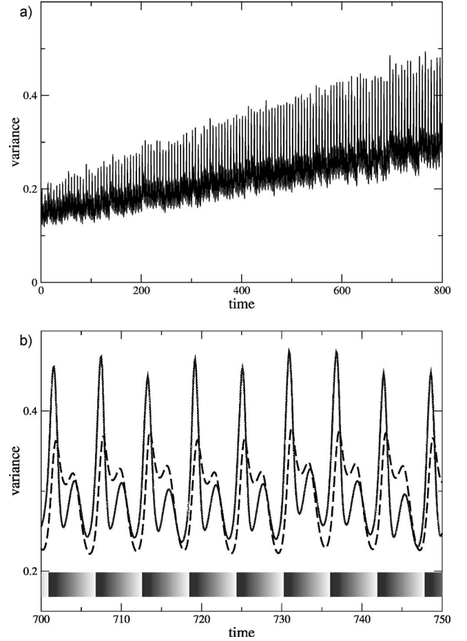
FIG. 3. (a) Variance evolution over a sample of 1000 independent Rössler systems. (b) Same as (a) within a time window of 700–750 (solid line). The dashed line indicates the modeled variance of the phase fluctuations. The mean phase of the oscillators is shown by the grey-scale strip on the lower part of the graph, ranging from 0 (black) to 2\pi (white).
