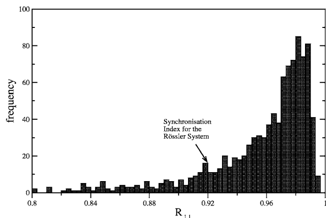
FIG. 4. Distribution of the synchronization index R_{1,1} for two independent processes of type (13). The parameters D , \Delta t , \omega and the amount of data N are chosen to allow a comparison of the results presented in Sec. III.
