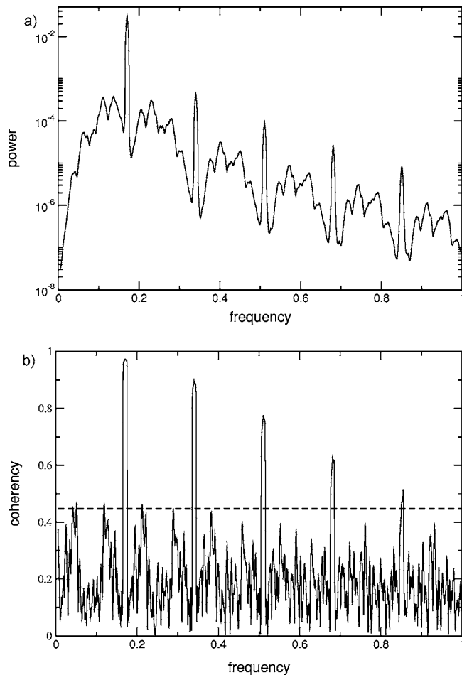
FIG. 1. (a) Power spectrum of the x component of the Rössler system at the vicinity of the main oscillating frequency. (b) Coherency of two independent, identical Rössler systems. The coherency at frequencies of approximately 0.17 and its multiples are lying above the 5% level of significance (dashed line).
